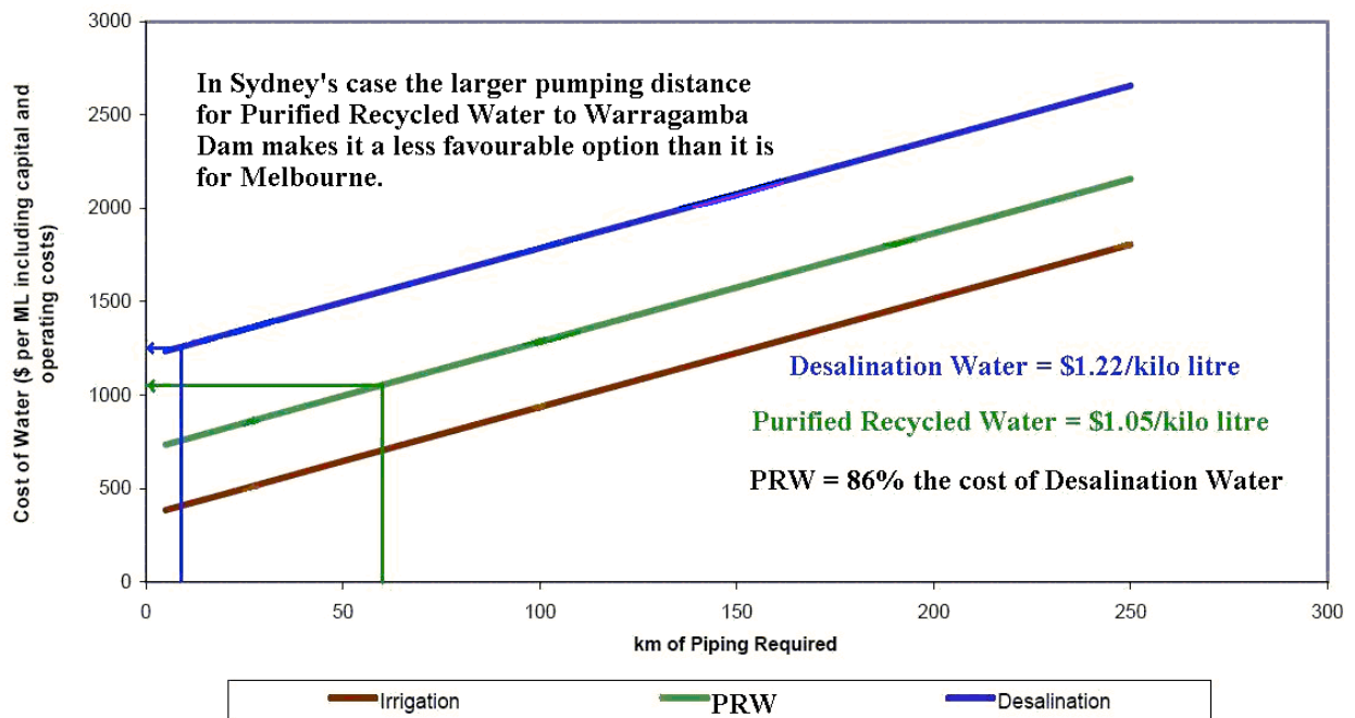
Figure 9: Comparison of water treatment costs and transport costs for a hypothetical case study to supply 100ML/day of an alternative water supply
